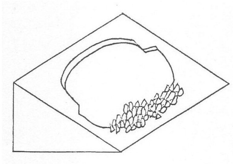
Figure 1.2: Slab Avalanche
