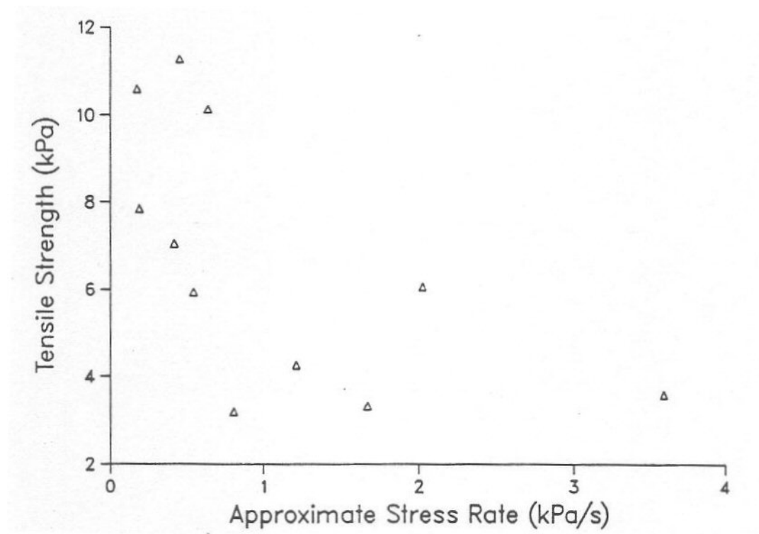
Figure 5.5: Effect of Stress Rate on Strength Eleven tensile tests made on a layer of rounded grains with a density of 298 \text{ kg/m}^3 at the Wolverine Study Plot on March 24, 1988.
