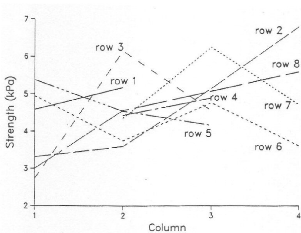
Figure 5.4: Strength Variation Within a Rectangular Subplot Twenty-four tensile tests of rounded snow with a density of 277 \text{ kg/m}^3 made in Wolverine Study Plot on March 2, 1988.
