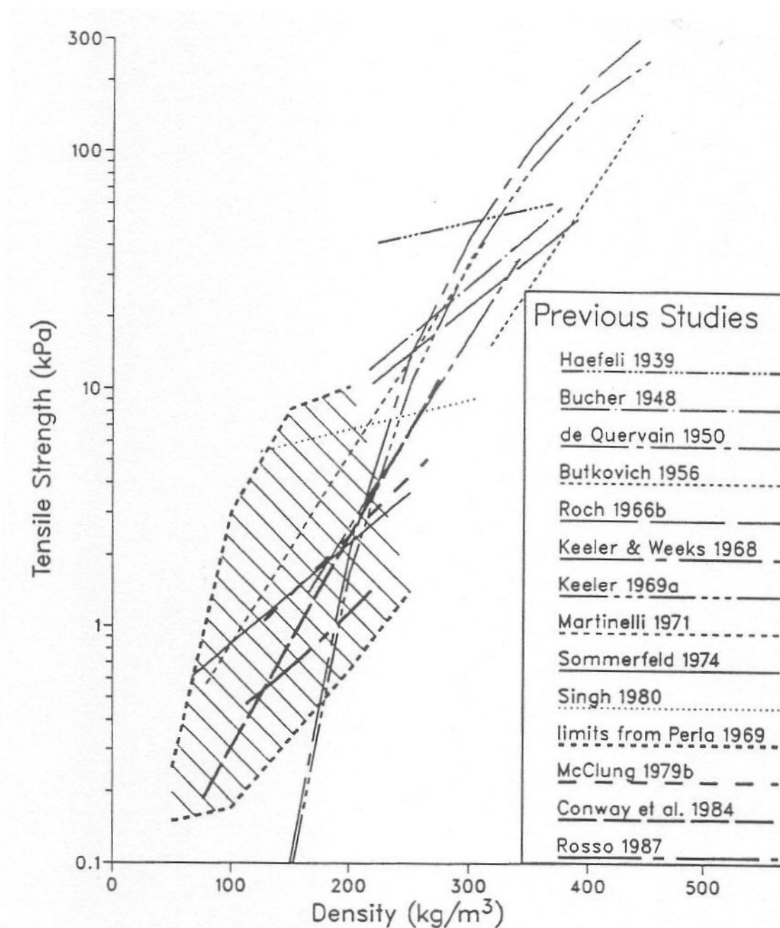
Figure 2.1: Tensile Strength from Laboratory and Field Studies
