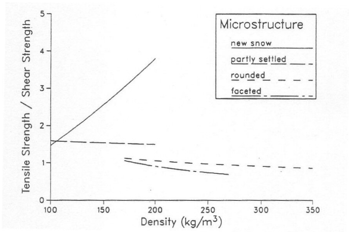
Figure 5.9: Ratio of Tensile Strength Regression to Shear Strength Regression for Four Types of Microstructure.
