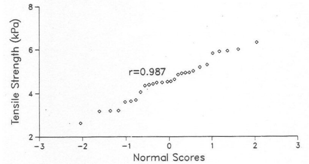
Figure 5.2: Normal Probability Graph of Sample of 42 Replicates. Tensile strength tests made on a layer of rounded snow with a density of 216 \text{ kg/m}^3 at Lipalian Study Plot on February 6, 1988.
