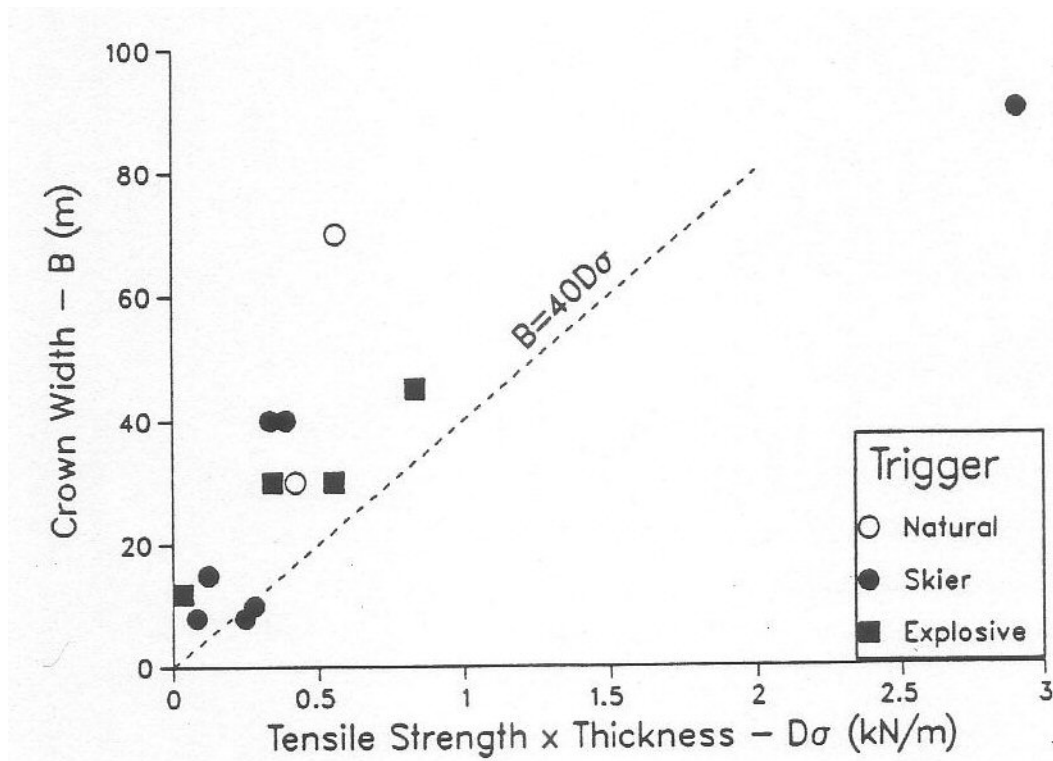
Figure 6.5: Crown Width vs Slab Thickness x Strength For 13 unconfined slab avalanches which occurred between January 25, and April 8, 1988 in and near the Lake Louise Ski Resort.
