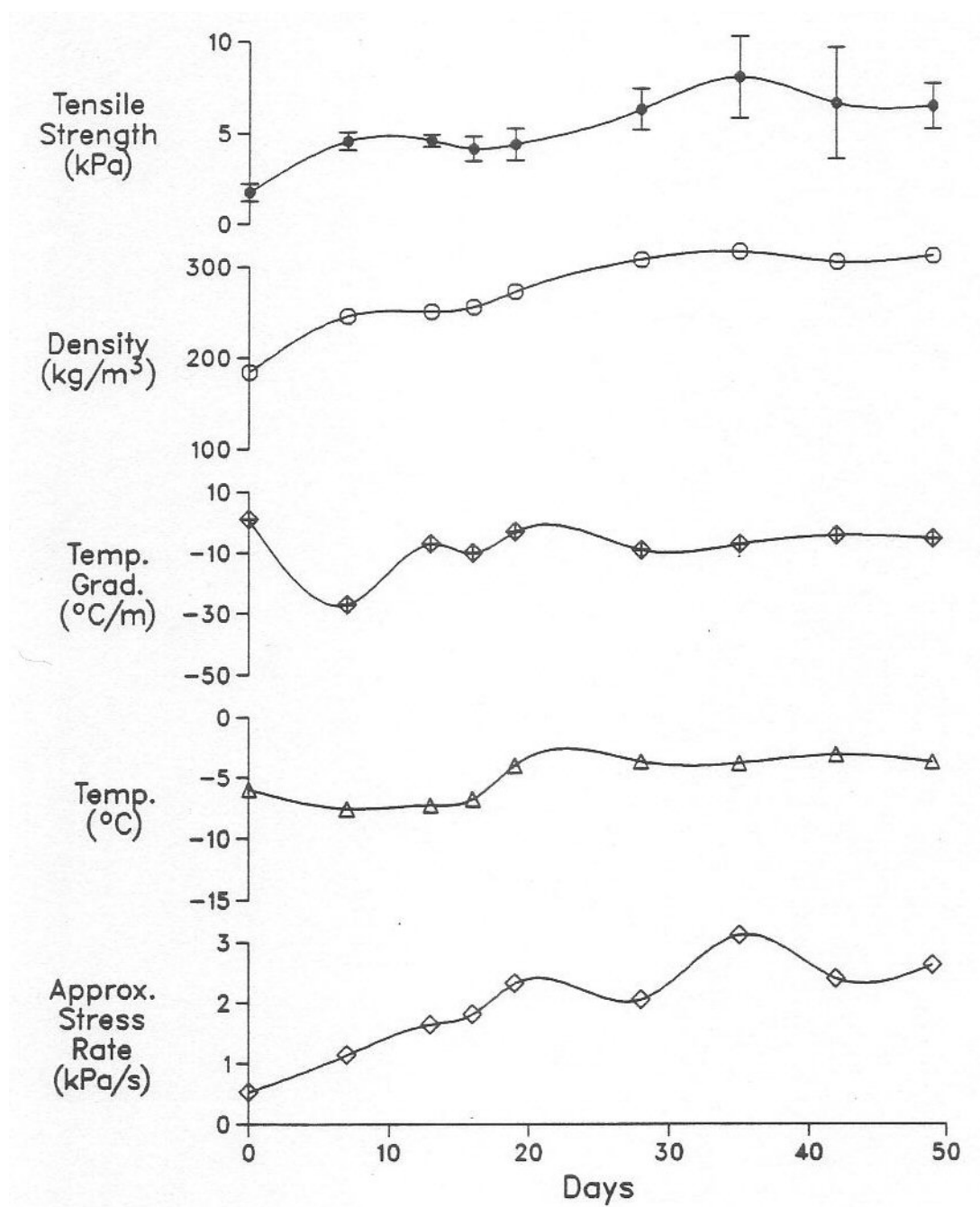
Figure 6.2: Tests of a Layer of Rounded Grains at the Richardson Plot Between Jan. 25 and Feb. 1, 1988.
