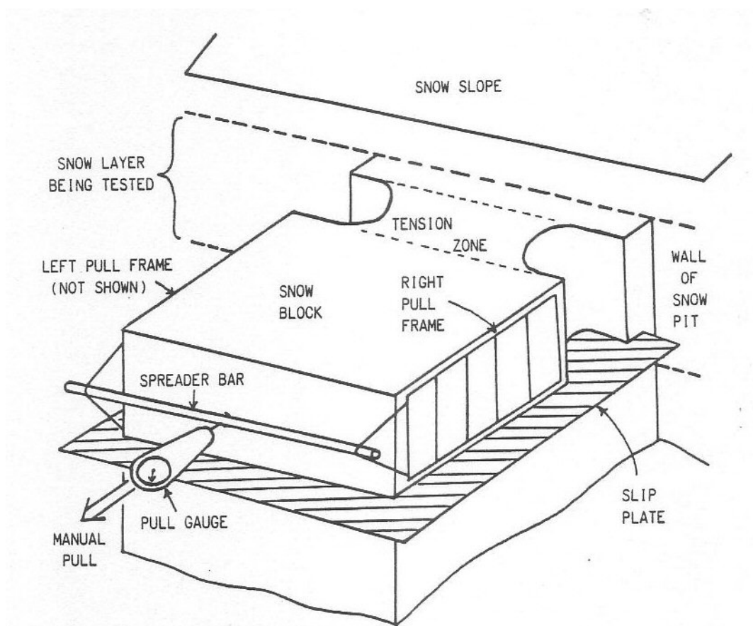
Figure 3.1: Slip Plate Tensile Test
